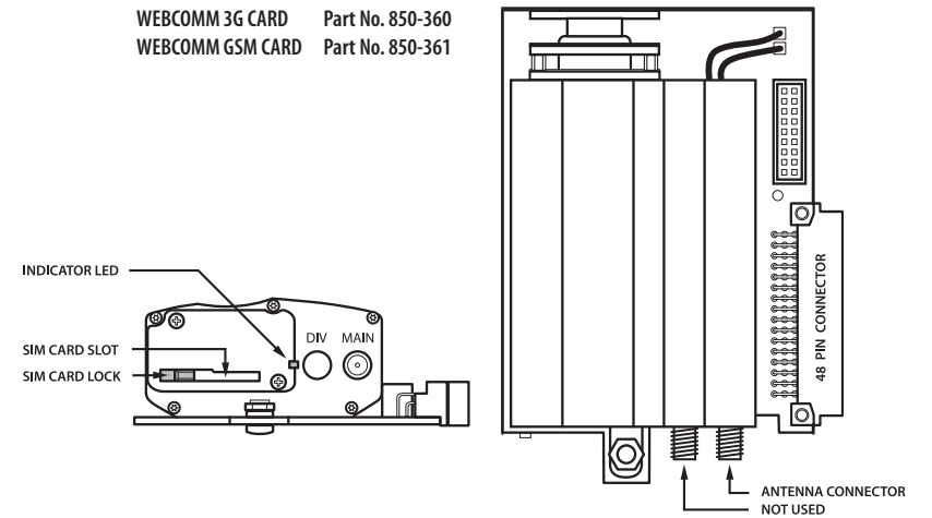
WEBCOMM 3G CARD Part No. 850-360
