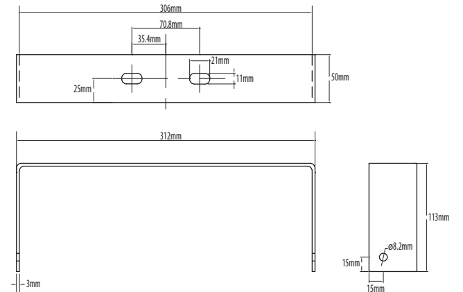
Mounting Kit - Solar Panel Bracket (Aluminium)
