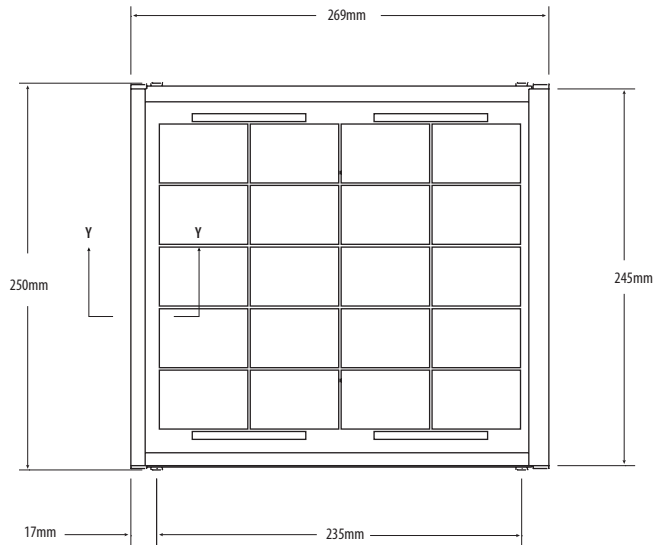
Solar Panel - Front View
