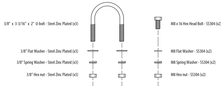
Mounting Kit - Fittings
