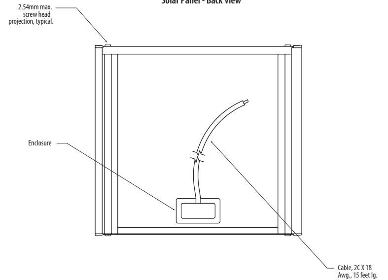
Solar Panel - Back View
