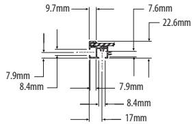
Solar Panel - Section Y-Y
