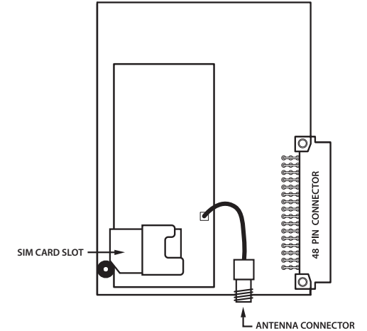
WEBCOMM 3G CARD Part No. 850-360
