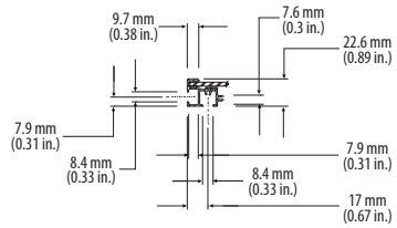
Solar Panel - Section Y-Y
