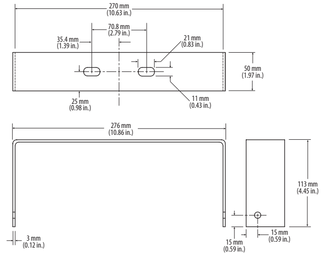
Mounting Kit - Solar Panel Bracket (Aluminium)
